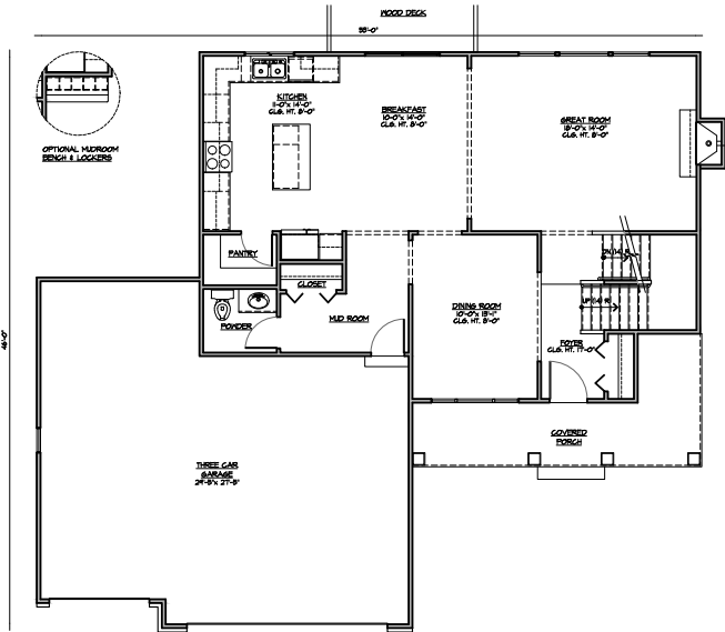
MAIN FLOOR PLAN 18' x 17'
