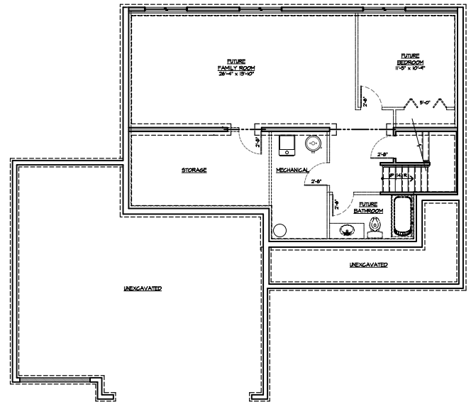
LOWER LEVEL FRAMING PLAN 18' x 17'
