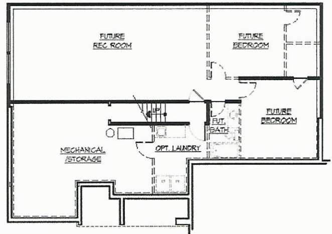
DAYLIGHT BASEMENT
