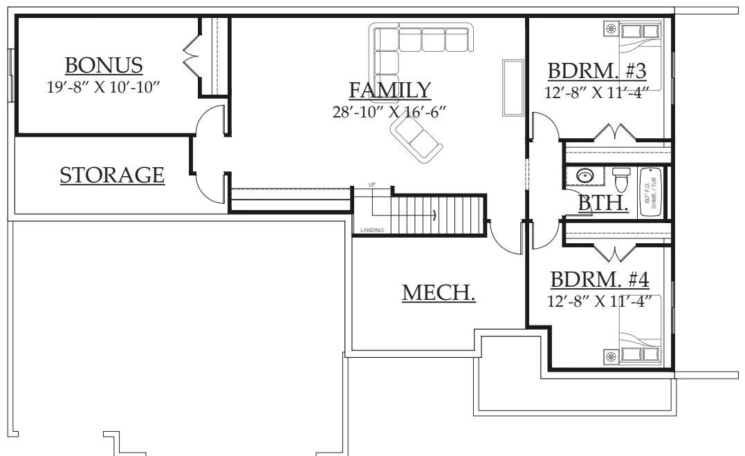
BASEMENT FLOOR PLAN 1,302 SQUARE FEET
