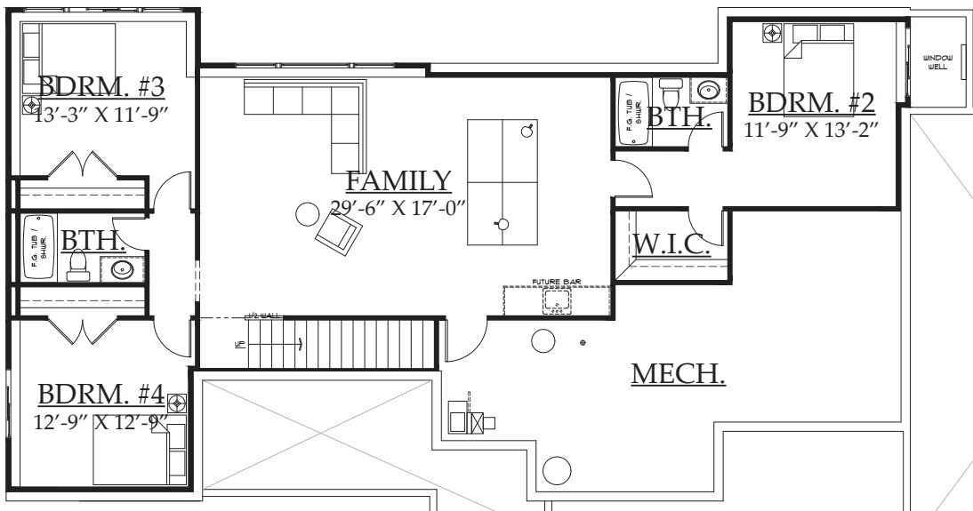
BASEMENT FLOOR PLAN 1,312 SQUARE FEET
