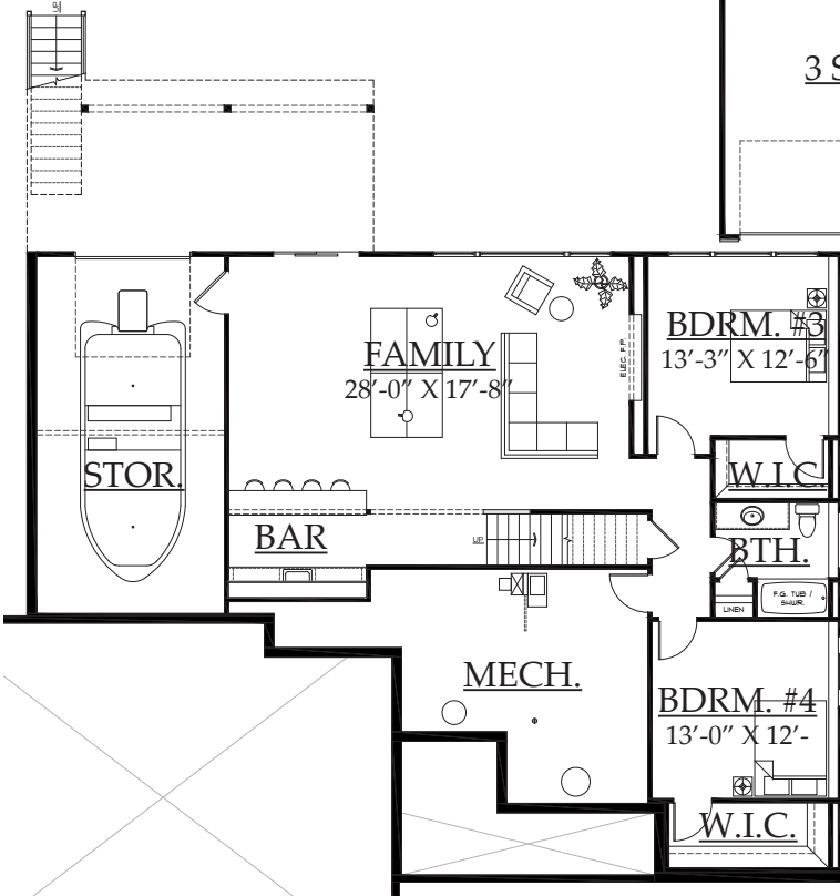
BASEMENT FLOOR PLAN 1,219 SQUARE FEET
