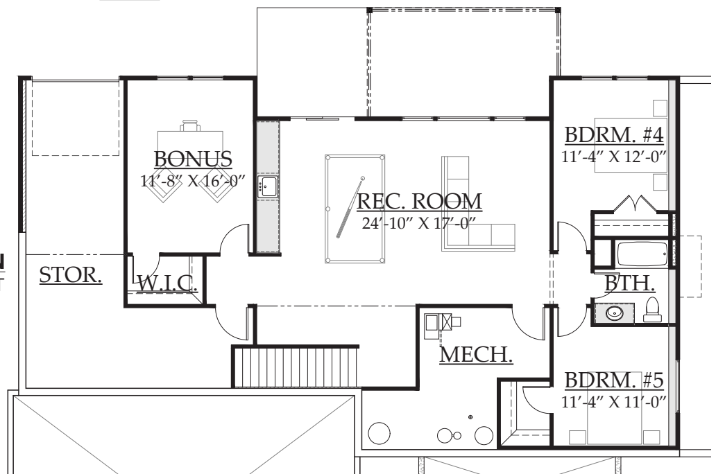
SECOND FLOOR PLAN 1,271 SQUARE FEET
