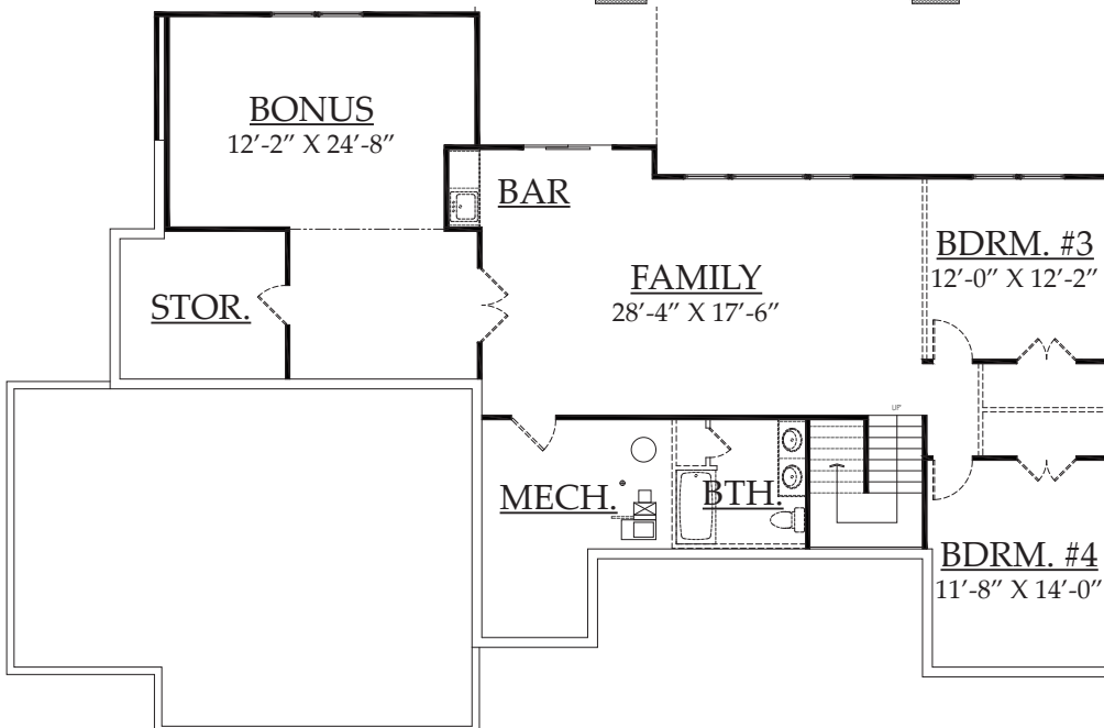
BASEMENT FLOOR PLAN 1,473 SQUARE FEET
