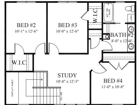
SECOND FLOOR PLAN 858 SQUARE FEET
